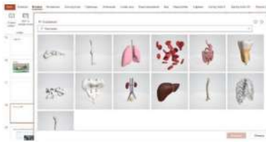
Рис. 5. Power Point 365
